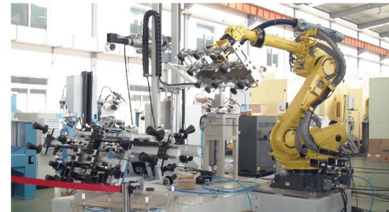
风挡涂胶 Windshield sealing robot
